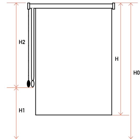
CADENA O CORDÓN CON TENSOR CORD OR CHAIN WITH COUNTERWEIGHT
